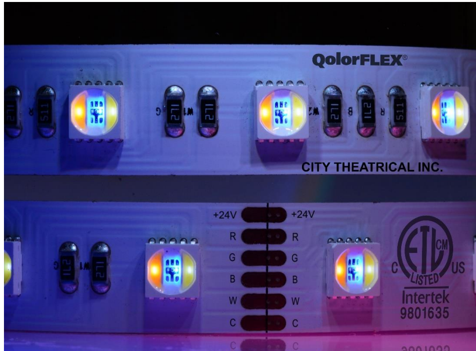
City Theatrical's QolorFLEX 5-in-1 HiQ High CRI LED Tape (top) vs. QolorFLEX 5-in-1 LED Tape RGBACW (below).
