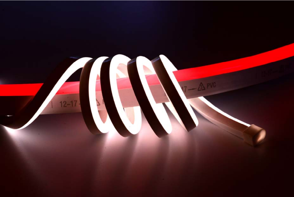
QolorFLEX NuNeon has a 12mm (0.5") minimum bending radius, making it up to 80% more flexible than similar products.
