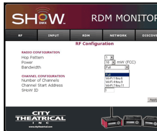
These two screen shots of SHoW DMX's built in RDM Monitor show how power and number of channels broadcast can be varied to decrease the effect on WiF
