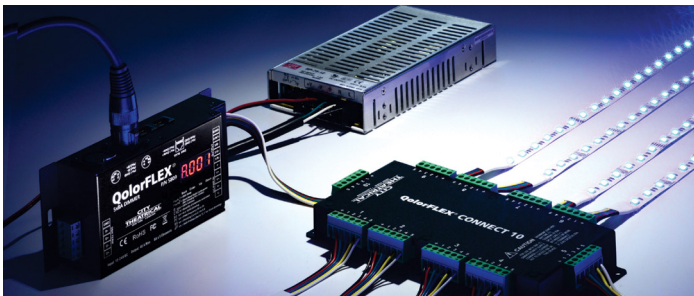
QolorFLEX 5x8A Dimmer (left) shown as part of a QolorFLEX installation.
