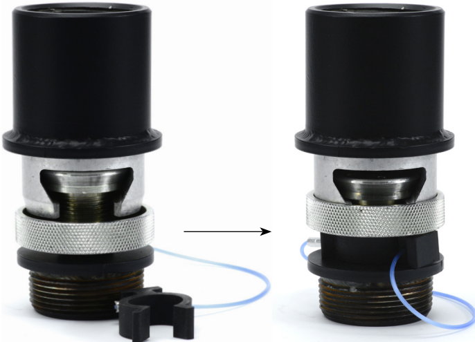
The one motion lock-in mechanism eliminates the need to manually twist heavy projectors to connect them to vertical pipes.
