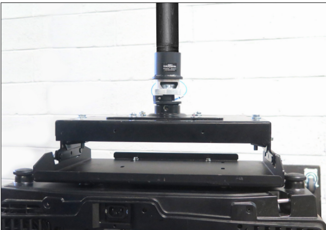
The Projector Hanger's Tee Slot System allows the user to slide the Tee Head, which attaches to the top of the projector, into the Tee Slot, which mounts at the end of a 1½" pipe.
