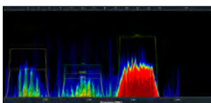
Spectrogram
